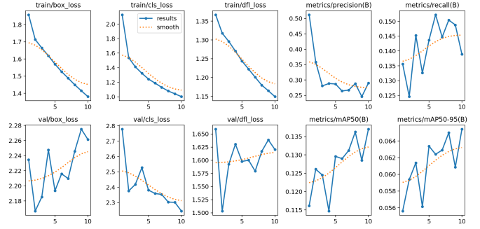
Fig. 7: YOLOv11n C_1 Boston fine-tune training curves.
